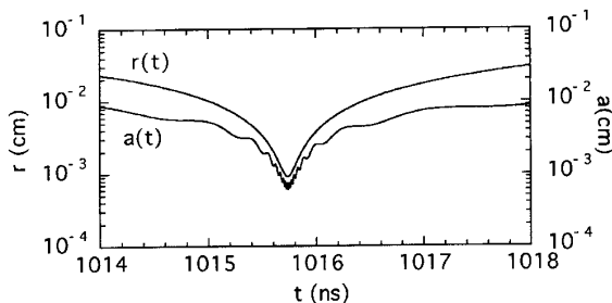
FIG. 3. Plots of the outer pinch radius and the inner fiber radius as a function of time during the last phase of compression.
