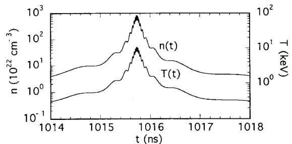
FIG. 5. Plots of the density and temperature of the fiber plasma as a function of time.
