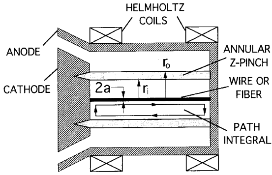
FIG. 1. Schematic illustration of the staged Z-pinch configuration.
