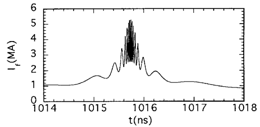
FIG. 4. Plot of the current through the fiber as a function of time.
