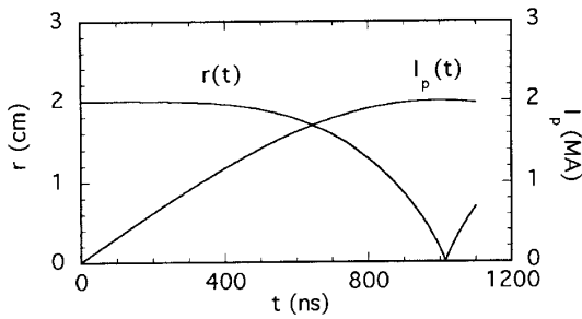
FIG. 2. Outer pinch current and outer pinch radius as a function of time.
